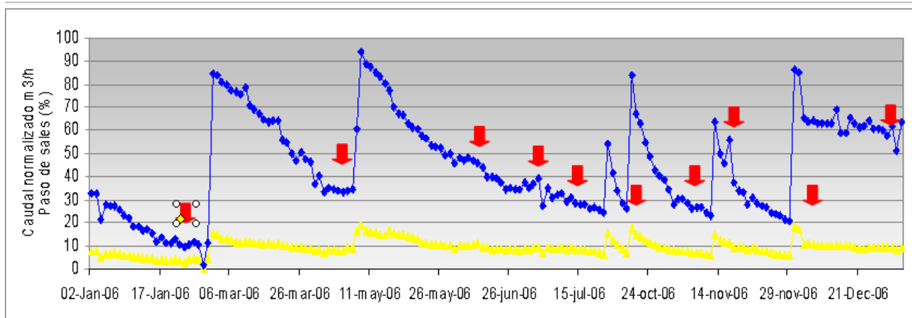
Figure 3.- Normalized permeate flux ( \text{m}^3/\text{h} ), rack 1, second stage. Chemical cleaning frequency.
