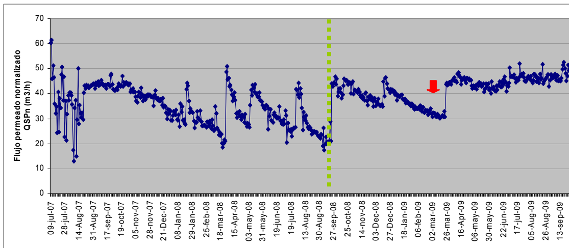
Figure 7.- Normalized permeate flow (m 3 /h) in stage 2 - Rack 1 (July 2007 – October 2009)
