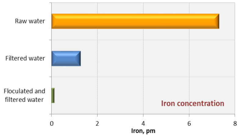
Figure 4.- Iron concentration during filtration process with and without flocculant (Genefloc GPF)
