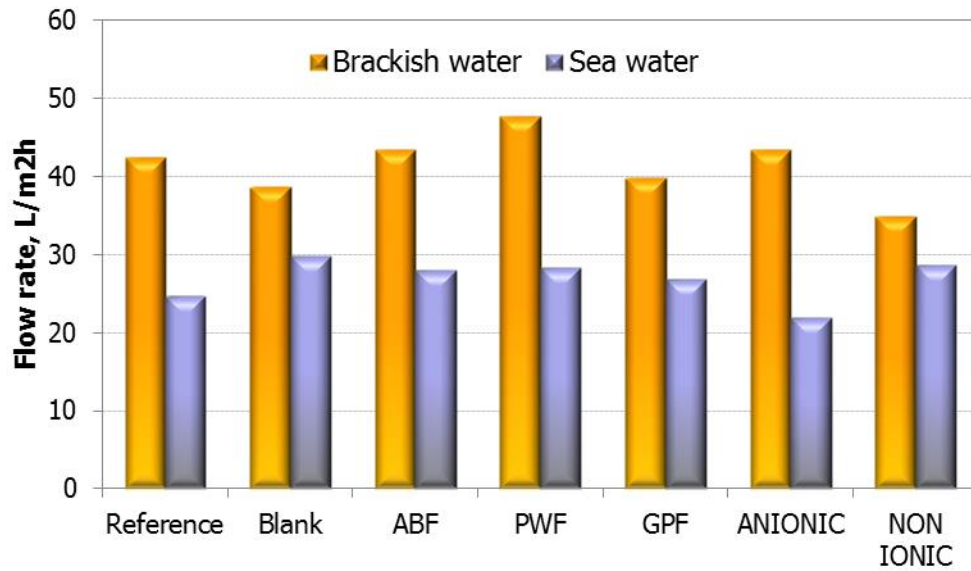
Figure 9.- Permeate flow rate performance parameters after soaking period in 1g/L flocculant solution
