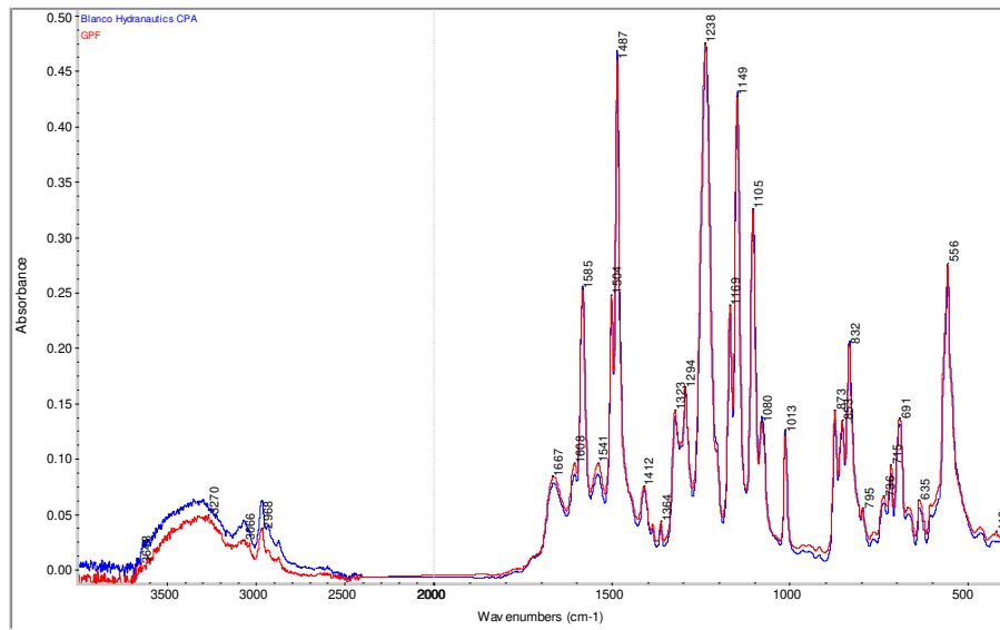
Figure 14.- Comparison of GPF coupon after soaking period to blank membrane spectra (brackish water)
