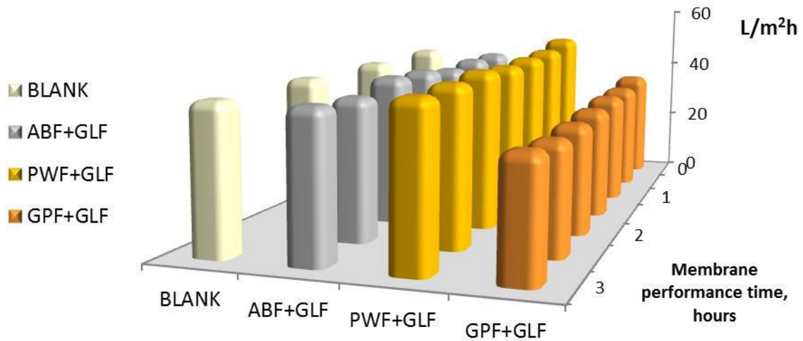
Figure 22.- Permeate flow rate membrane performance after 100 ppm GLF and 100 ppm flocculants dose
