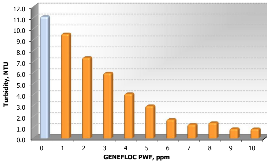
Figure 1.- Turbidity values obtained after Genefloc PWF dosing and later filtration
