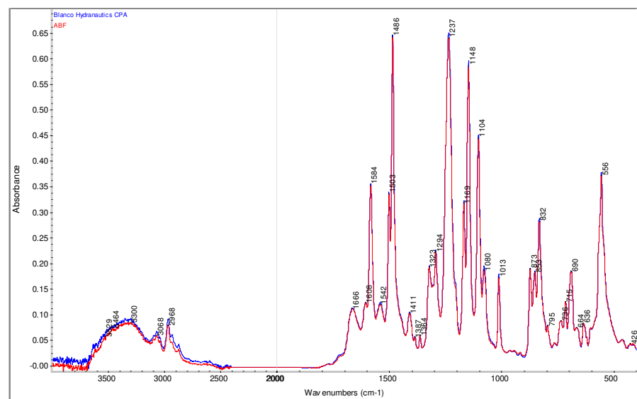
Figure 15.- Comparison of ABF coupon after soaking period to blank membrane spectra (brackish water)
