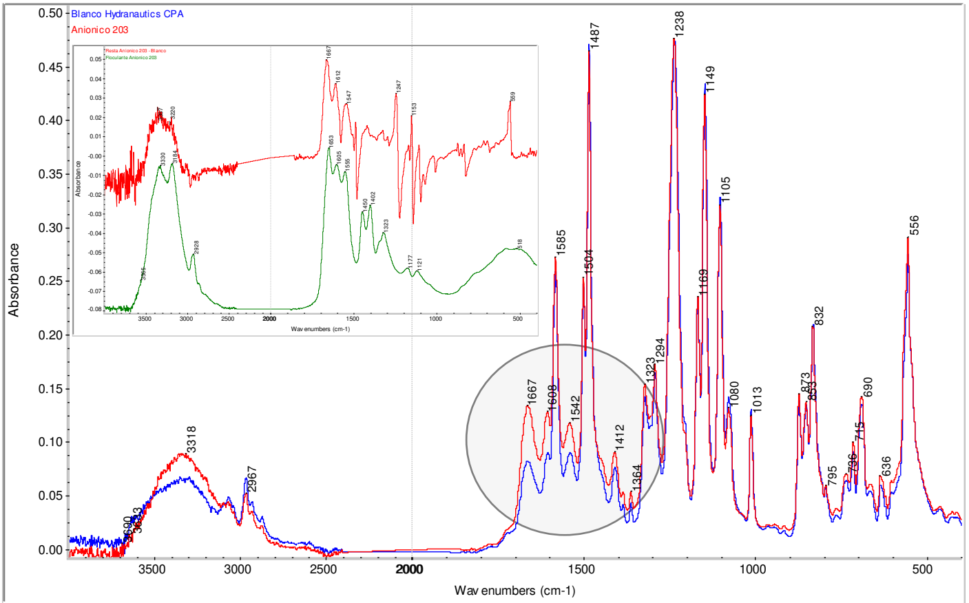
Figure 11.- Comparison of anionic coupon after soaking period to blank membrane spectra (brackish water)
