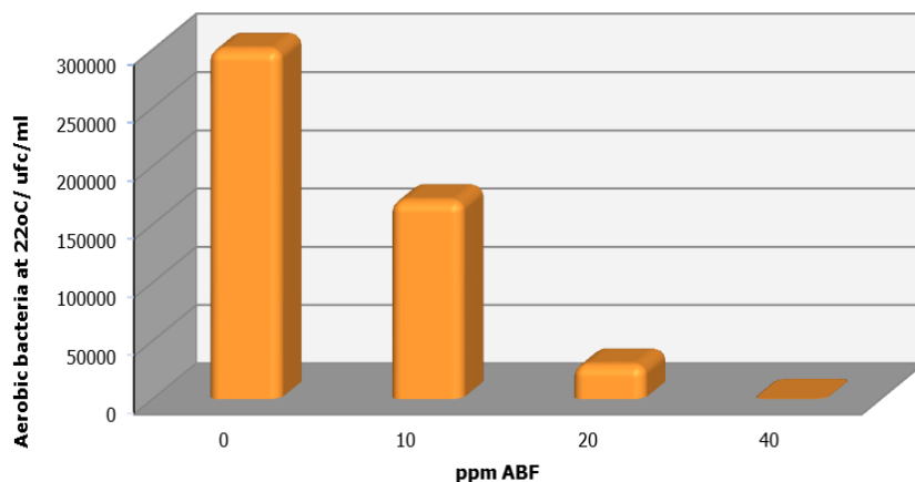
Figure 8.- Genefloc ABF activity against aerobic bacteria
