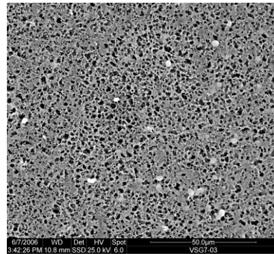
Microphotograph 6.- SDI filter obtained after 5 ppm flocculant dosing. SDI value: 4.3
