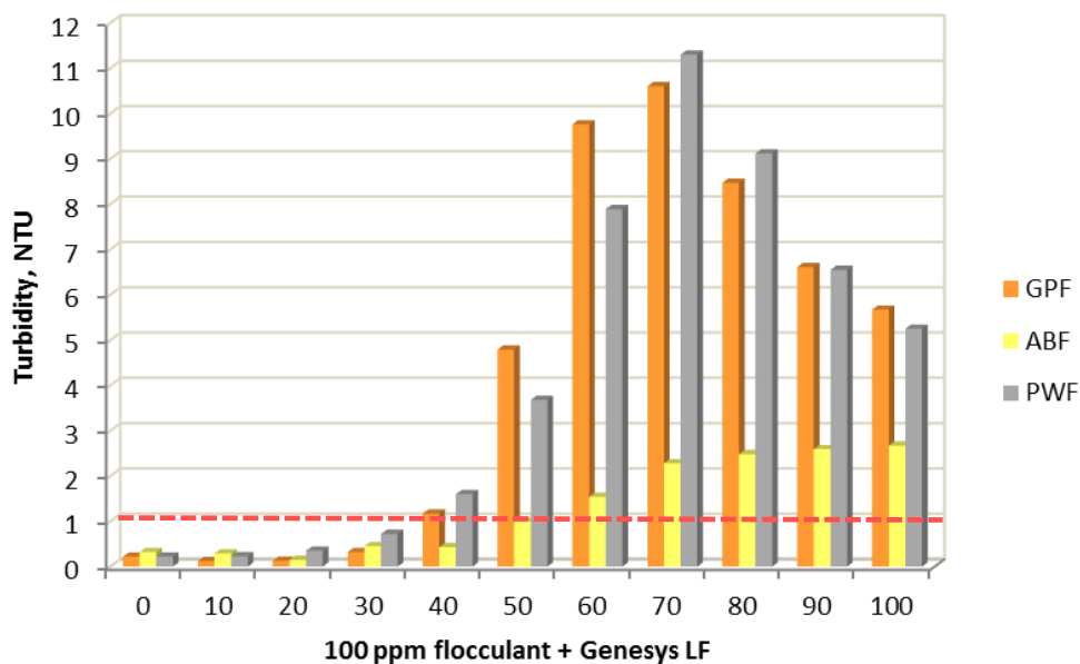
Figure 19.- Turbidity changes after Genesys LF dosing on a 100 ppm of flocculant solution -demin water
