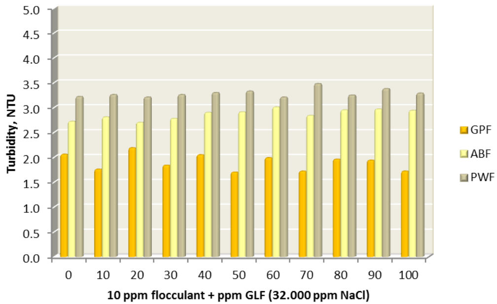
Figure 20.- Turbidity changes after Genesys LF dosing on a 10 ppm of flocculant solution – sea water
