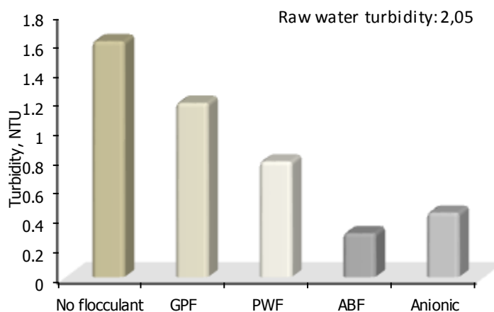
Figure 7.- Filtered water samples turbidity after different flocculants dosing
