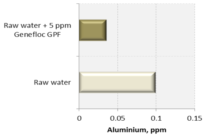
Figure 5.- Aluminium concentration during filtration process with and without flocculant (Genefloc GPF)
