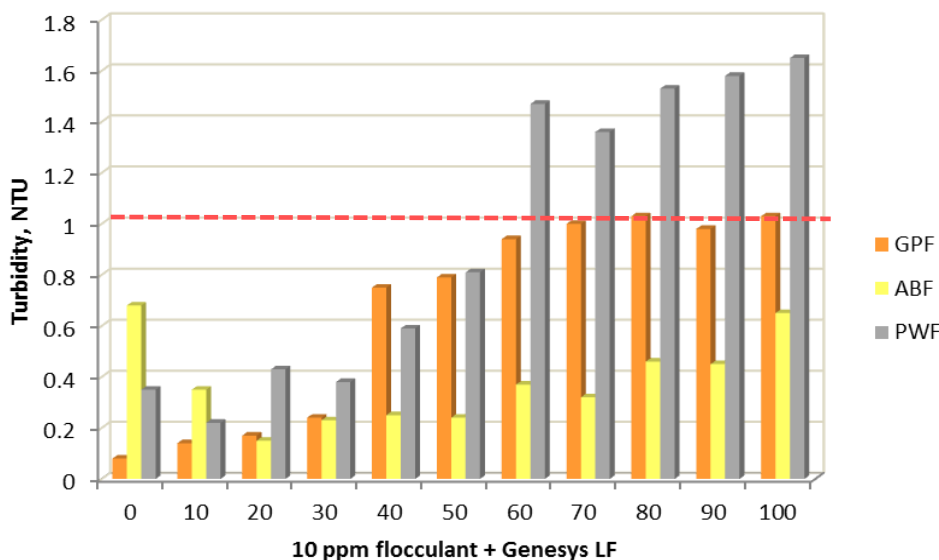
Figure 18.- Turbidity changes after Genesys LF dosing on a 10 ppm of flocculant solution-demin water
