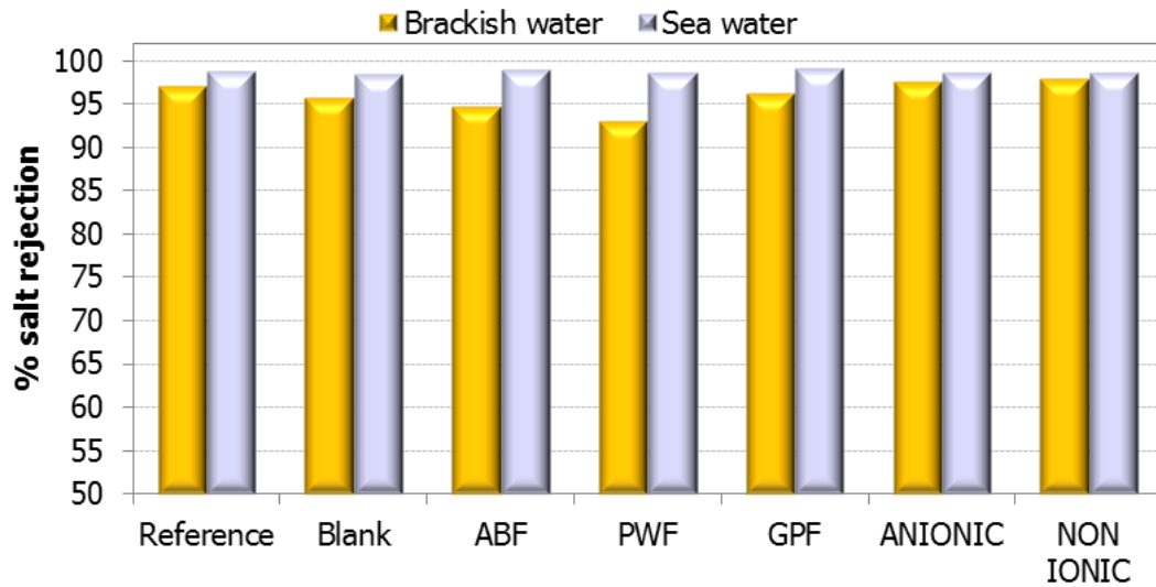
Figure 10.- Salt rejection percentage performance after soaking period in 1g/L flocculant solution
