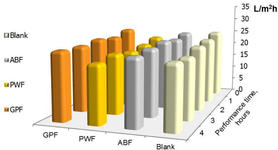
Figure 17.- Sea water membrane performance after flocculant dosing
