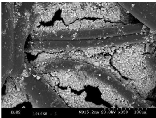
Microphotographs 1.- Cartridge filters fouled by aluminosilicates / colloidal matter
