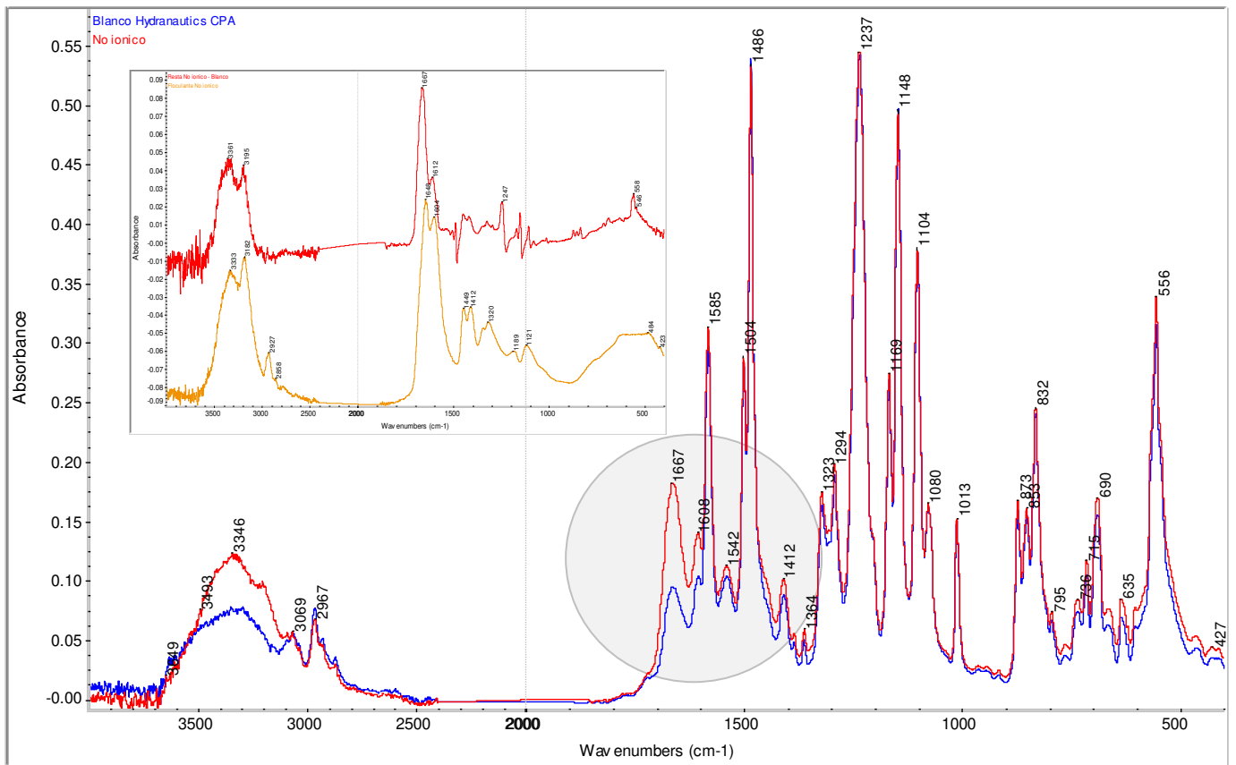
Figure 12.- Comparison of non ionic coupon after soaking period to blank membrane spectra (brackish water)
