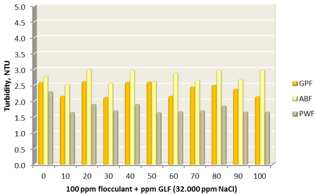
Figure 21.- Turbidity changes after Genesys LF dosing on a 100 ppm of flocculant solution – sea water
