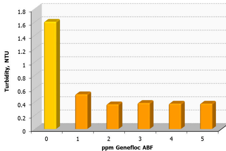
Figure 6.- Filtered water sample turbidity after different Genefloc ABF dosing
