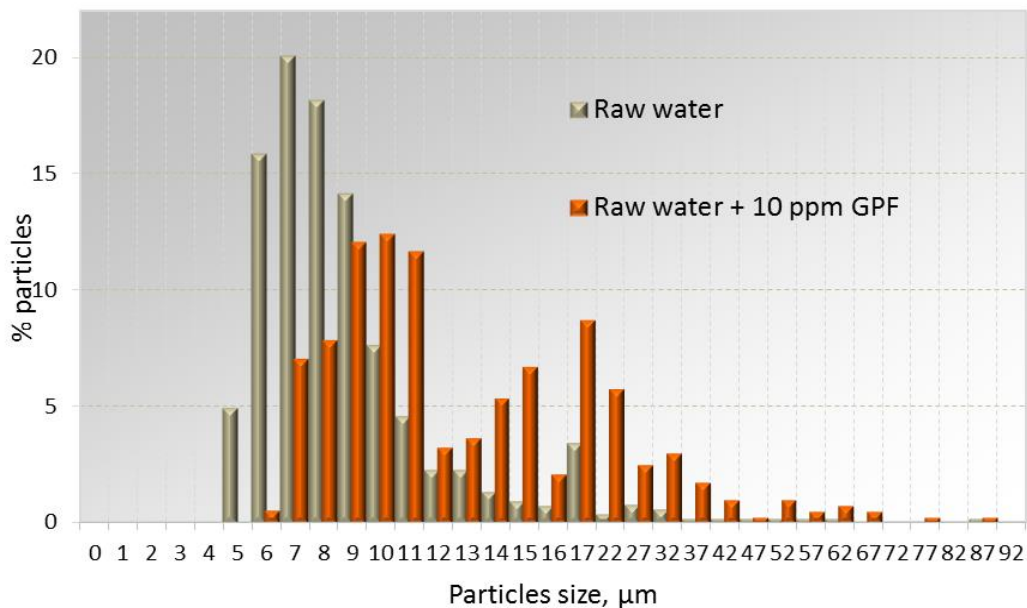
Figure 3.- Particle size distribution of a water sample after additional dosage of flocculant
