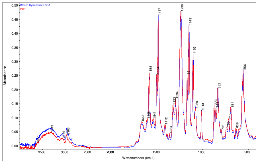
Figure 13.- Comparison of PWF coupon after soaking period to PWF flocculant spectra (brackish water)
