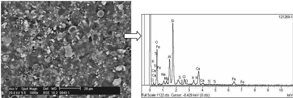
Microphotograph 7.- SEM image of an SDI disk completely covered by aluminosilicates (clay/colloidal matter)
