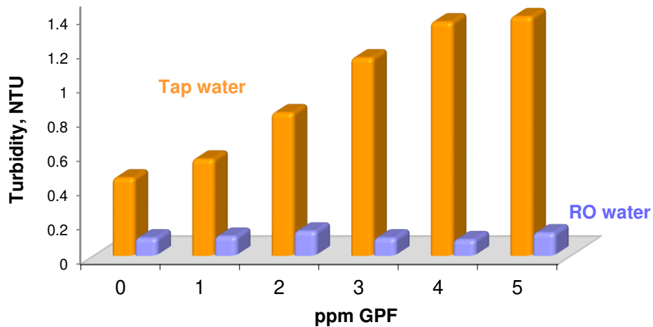
Figure 2.- Turbidity values of a tap water sample after flocculant dosage, compared to a RO water with no particles
