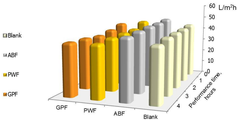
Figure 16.- Brackish water membrane performance after flocculant dosing
