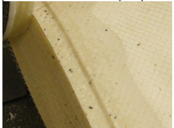
Photograph 6.- Presence of corrosion drags on membrane surface - feed side
