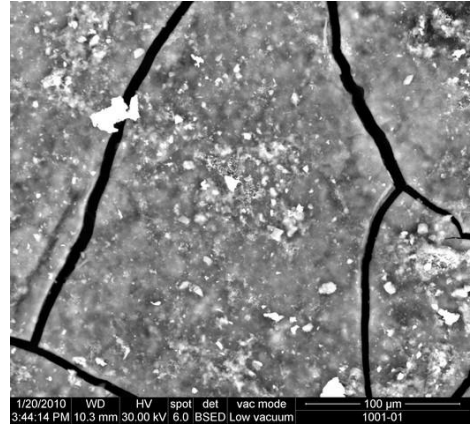
Photograph 4.- Detail of fouling with iron, which corresponds to the brighter component. Iron commonly appears at SEM as very bright and tiny particles mixed with the rest of components
