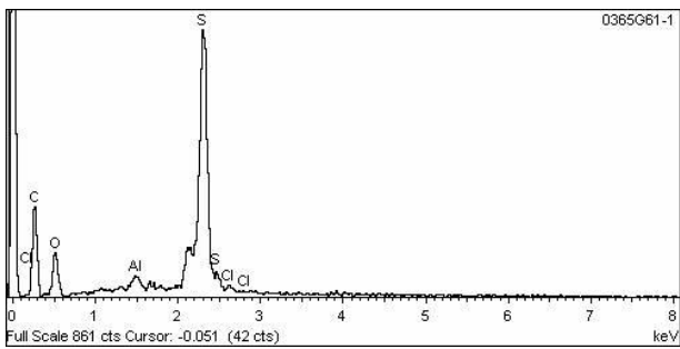
Figure 25. EDX results obtained from PES fiber after cleaning with neutral cleaner
