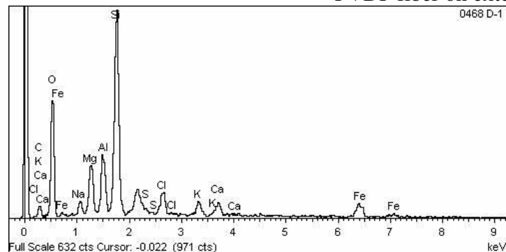
Figure 21. EDX results obtained from PVDF fiber fouling
