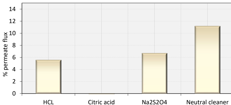
Figure 6. Permeate flux improvement percentage obtained during cleaning tests for iron removal.
