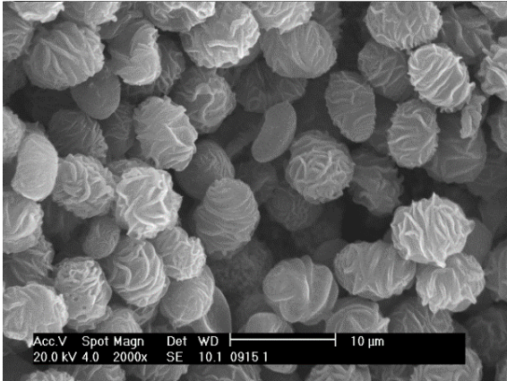
Photograph 3.- Detail of iron particles Granular shape
