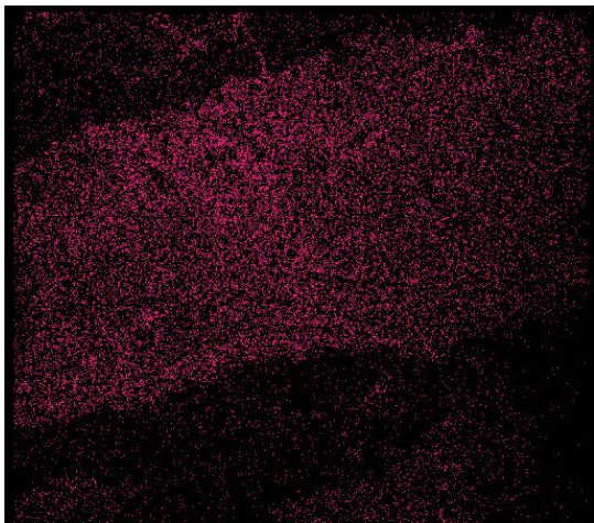
Figure 12. Distribution of aluminium on membrane surface after cleaning with AC-3 (mild acid)
