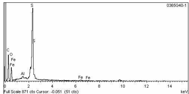
Figure 26. EDX results obtained from PES fiber after cleaning with ALK-1
