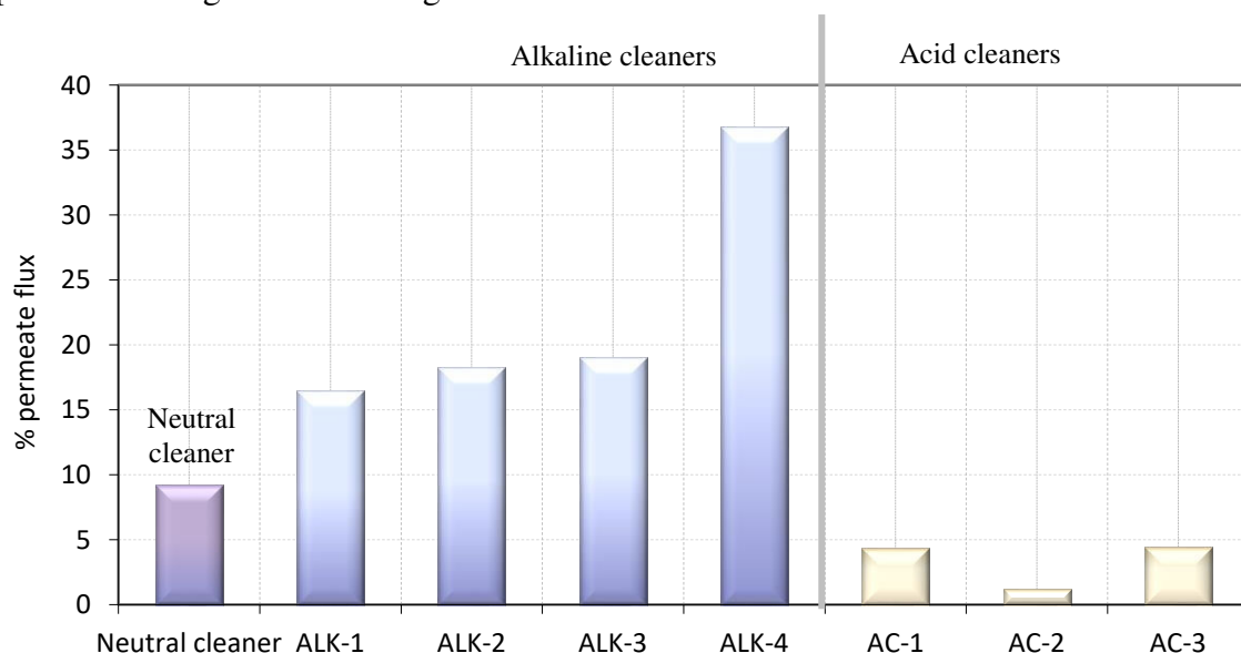
Figure 11. Permeate flux improvement percentage obtained during cleaning tests for aluminium removal
