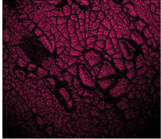
Figure 11. Distribution of aluminium on membrane surface
