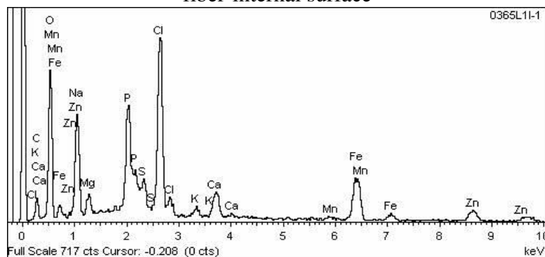
Figure 24. EDX results obtained from PES fiber fouling
