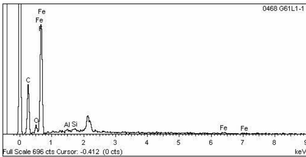
Figure 22. EDX results obtained from PVDF fiber after cleaning with neutral cleaner
