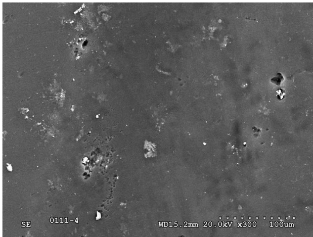
Photograph 17.- Abrasion marks from corrosion drags on membrane surface
