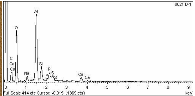
Figure 10. EDX results obtained from aluminium membrane fouling.
