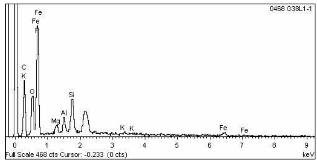
Figure 23. EDX results obtained from PVDF fiber after cleaning with AC-2
