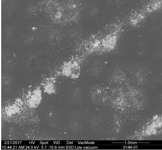
Photograph 20. Fouling composed of iron and aluminosilicates was concentrated on spacer support areas of membrane surface.
