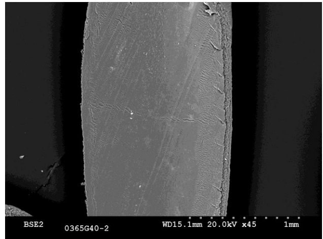
Photograph 40.- Detail of PES fiber after cleaning with ALK-1 (alkaline cleaner)
