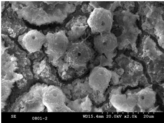
Photograph 13.- Detail of manganese fouling. Manganese commonly shows very characteristic spherical structures mixed with the rest of fouling components
