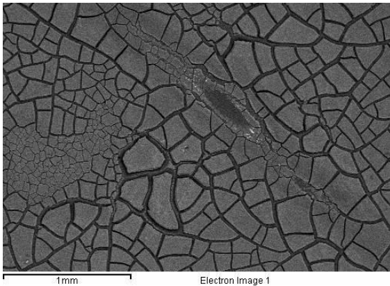
Photograph 9.- Detail of membrane surface with main presence of aluminium fouling. A cracked and thick fouling is characteristic of aluminium fouling.
