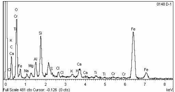
Figure 5. EDX results obtained from iron membrane fouling.
