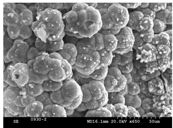
Photograph 16.- Detail of chromium fouling
