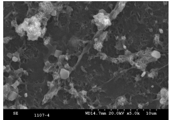
Photograph 14.- Detail of membrane surface with manganese fouling. It is common to find manganese structures dispersed on membrane surface.
