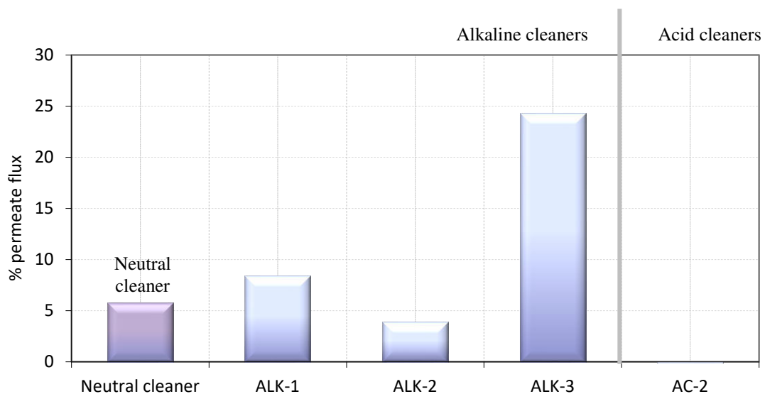
Figure 15. Permeate flux improvement percentage obtained during cleaning tests for manganese removal
