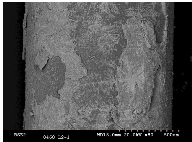
Photograph 31.- General view of fouling on PVDF fiber on external surface
