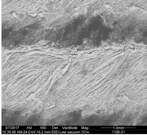
Photograph 26. General view of fouling on membrane surface
