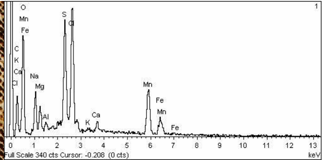
Figure 14. EDX results obtained from manganese membrane fouling.
