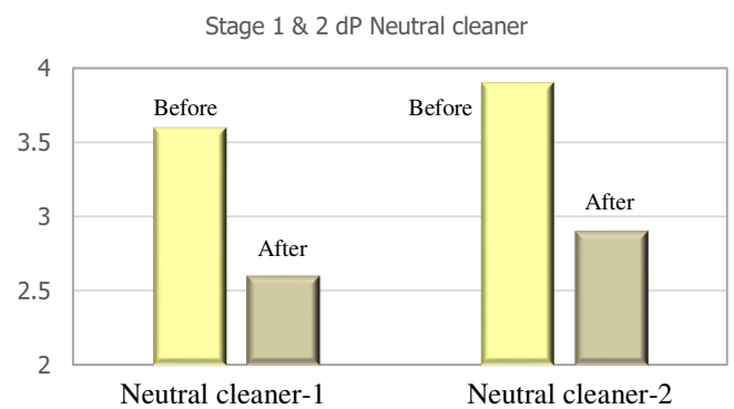
Figure 20.- Changes observed in dp after cleaning with neutral cleaner at stage 1 and 2
