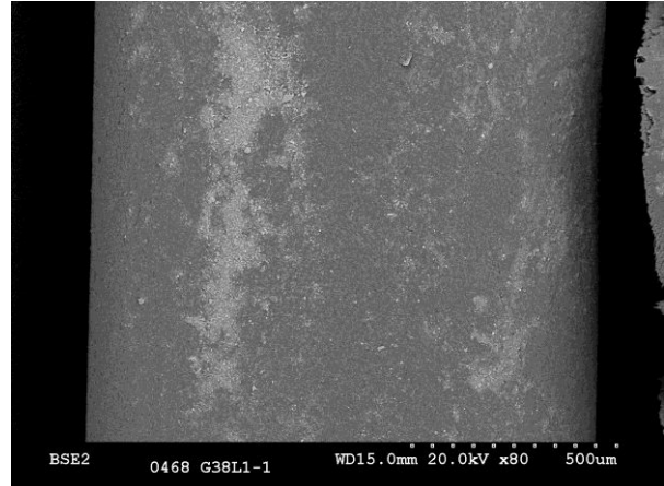
Photograph 34.- Detail of PVDF fiber after cleaning with AC-2 (acid cleaner)
