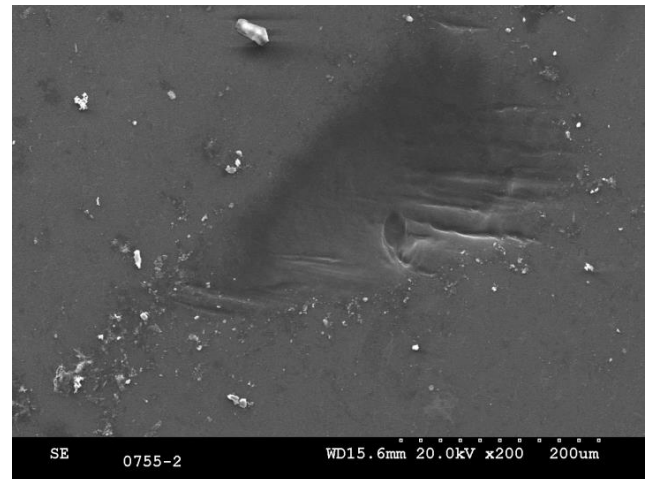
Photograph 18.- Abrasion marks from corrosion drags on membrane surface
