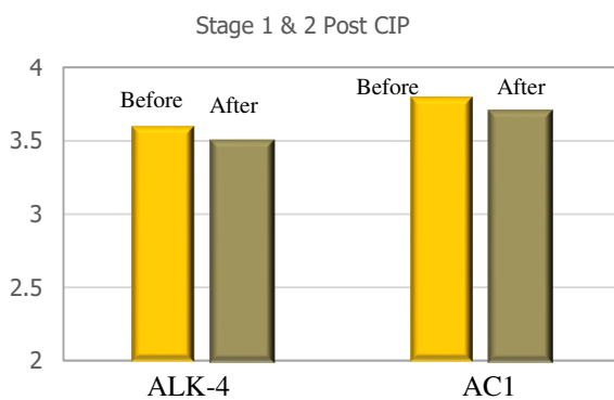
Figure 19.- Changes observed in dp after cleaning with ALK4 (stage 1) and AC-1 (stage 2)
