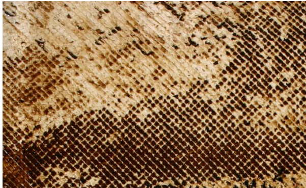
Photograph 25.- General view of membrane surface with presence of manganese
