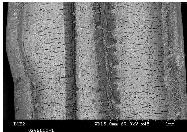
Photograph 37.- General view of fouling on PES fiber-internal surface
