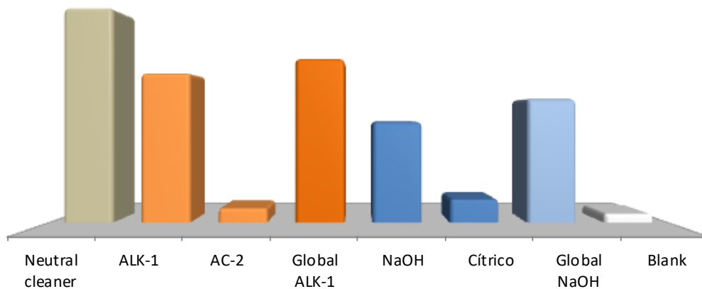
Figure 27.- Percentage flux increase obtained during cleaning tests carried out with PES fibers
