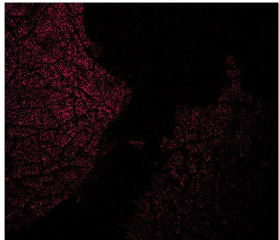
Figure 13. Distribution of aluminium on membrane surface after cleaning with neutral cleaner
