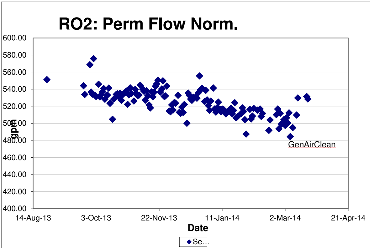
Figure 5: Graph of Normalised permeate flow over time and after Genairclean.
