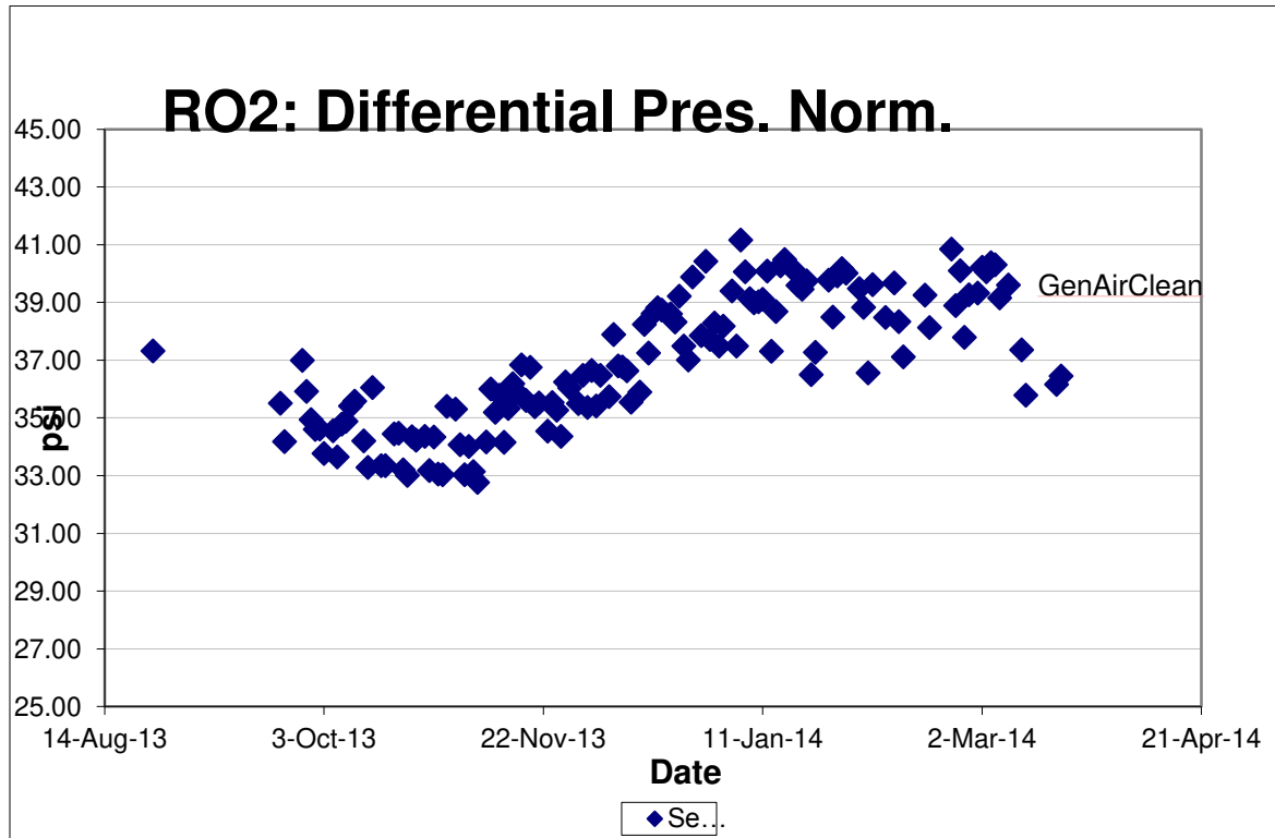
Figure 6: Graph of differential pressure over time and Genairclean.
