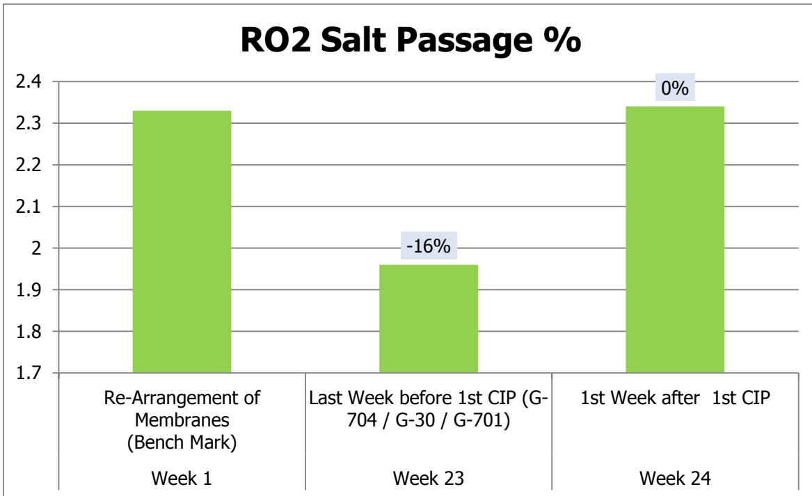
Figure 7: Graph of Salt Passage over time and Genairclean.
