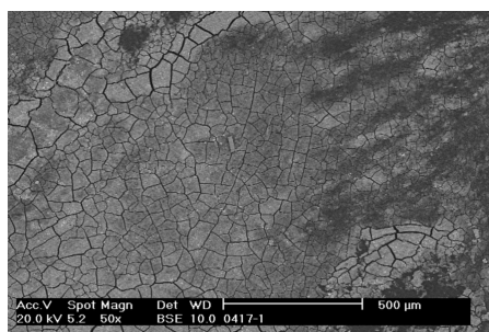
Figure 3: SEM Micrograph showing aluminosilicate deposit detail on RO membrane surface prior to cleaning with Genesol 703
