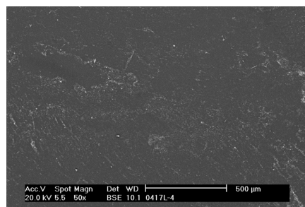
Figure 4: SEM Micrograph of same RO membrane surface after cleaning with Genesol 703 showing complete deposit removal
