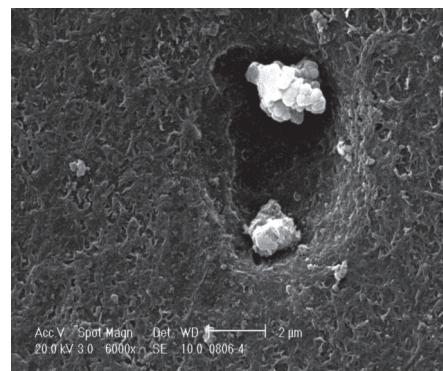
Figure 1: SEM-EDX membrane autopsy picture of aluminosilicates showing abrasion at the membrane surface
